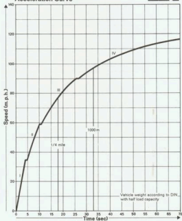
Acceleration Curve
