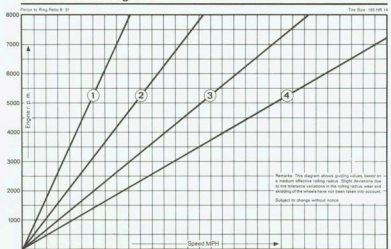
Transmission Diagram
