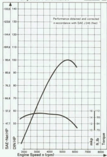
Full-power Performance
